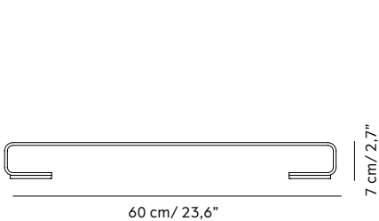
TOWELBAR, BLACK, WHITE Category: Towel Bar H: 3,5 cm / 1,1", W: 60 cm / 23,6", D: 7 cm / 2,7"
